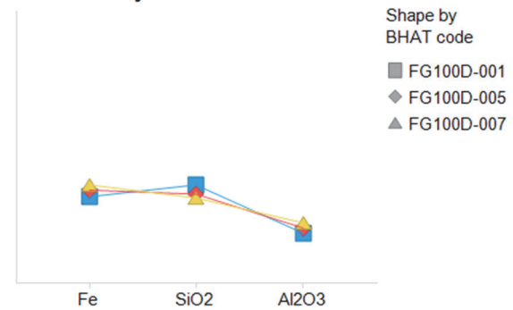
Figure 1. Summary results for different methods of assay data acquisition at a mining site (left). Note the high error for manual blastcone sampling using shovels and the lowest error for the BHAT method. The plot on the right shows field error for three BHAT units operating at the mine site, showing consistent results. Note: One Standard Error is given as the standard deviation of the absolute difference between sample pairs.
