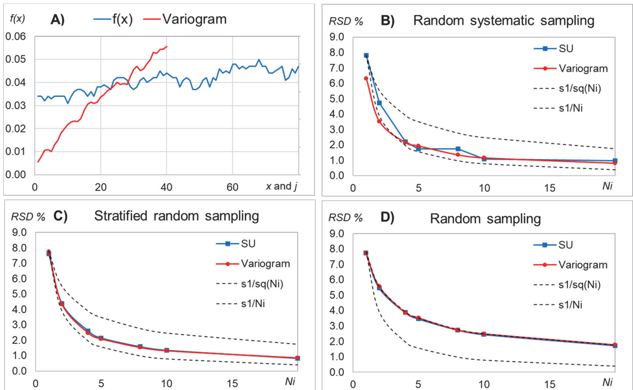
Figure 2. Influence of trends in data for predictions of sampling uncertainty (RSD %) for variogram integration and for SU estimation. A) Concentrations, f(x) , and variogram. Data from Pitard [2]. B) to D). Predicted RSD % from SU and variogram integration. The black dotted lines indicate the position for a RSD % proportional to 1/\sqrt{N_i} and 1/N_i .
