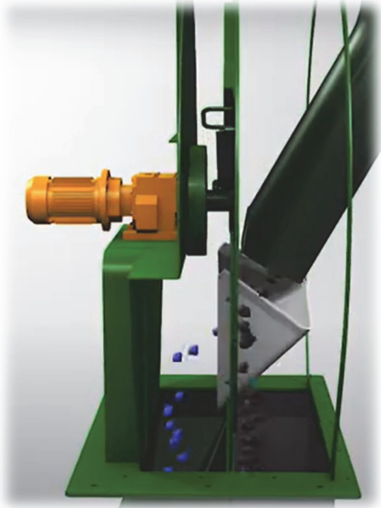
Figure 3. Sectional view of the Rotating Plate Divider feed pipe (on the right) presenting a sample increment to the cutter (middle) to sub-sample (blue particles) the stream and generate rejects (black particles) on the feed side of the plate. Sample and rejects report to separate, isolated chutes.
