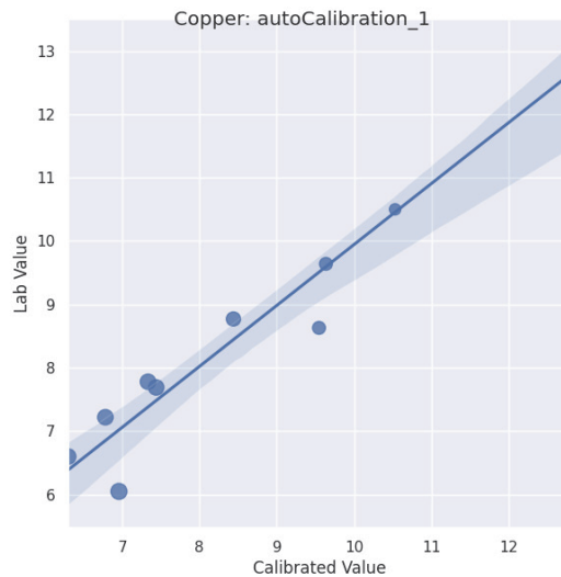
Figure 5. Cu calibration curve obtained with the training set of the measurements of ore slurries at GTK Mintec (MAPE = 5%, MAE = 0.36%).
