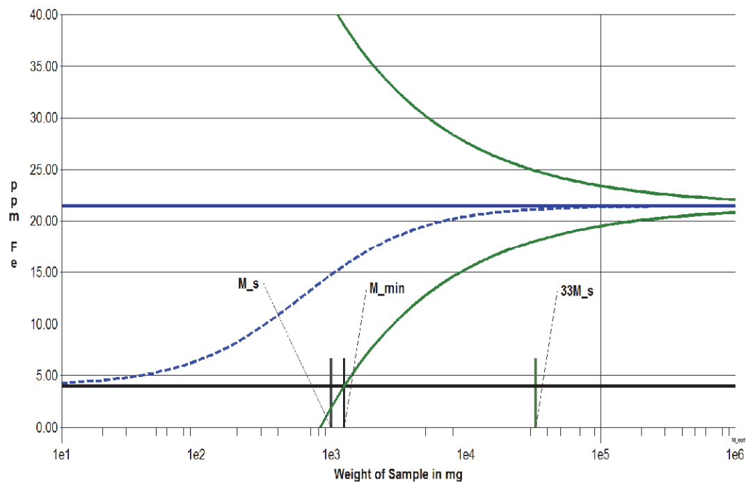
Figure 8. Illustration of the Ingamells' sampling diagram for ammonium paratungstate
