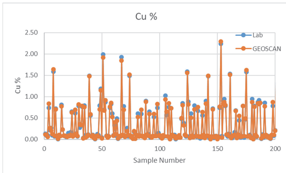
Figure 2. GEOSCAN and laboratory results for Cu %
