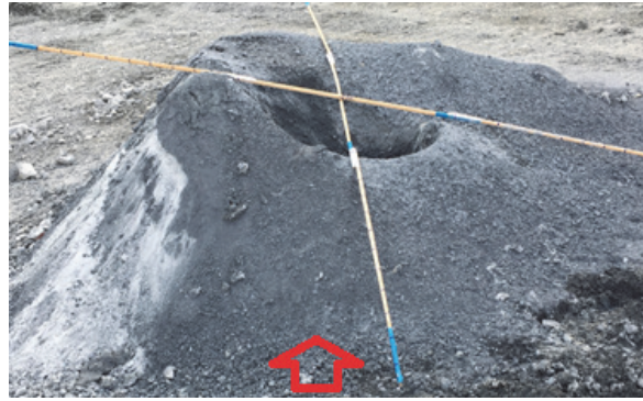
Figure 9. Material around rotary percussion drilling cone of blast hole (BH06) (looking towards drill rig). Note the irregular shape of drill chip cone.
