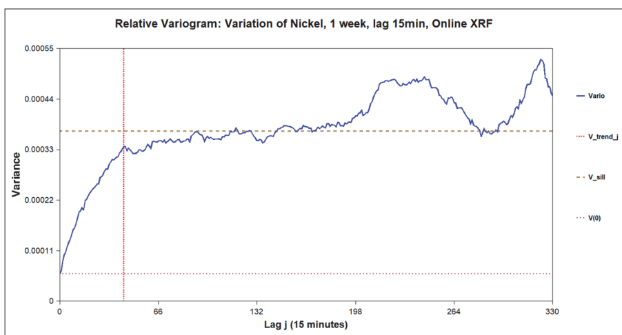
Figure 8: Relative variogram of Nickel measured by photometry
