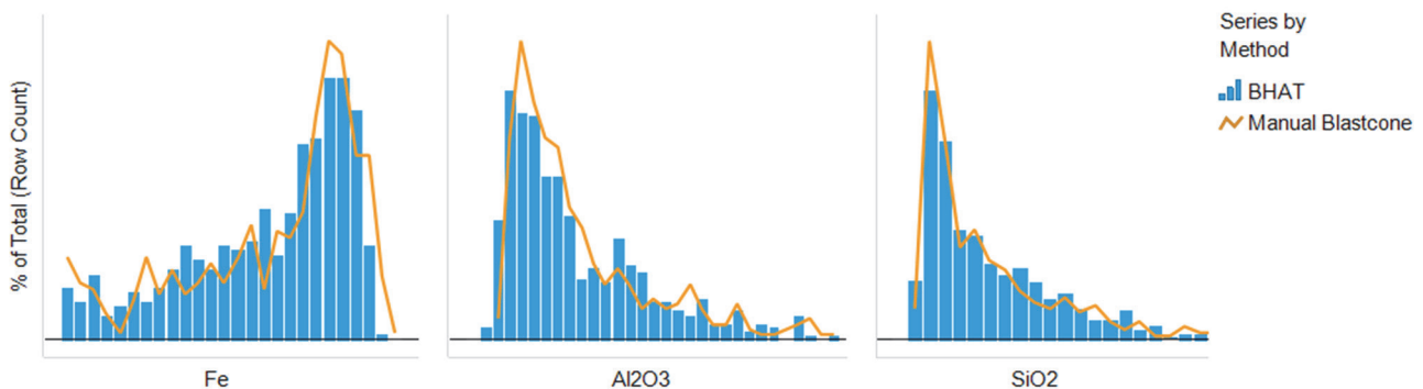
Figure 2. Illustration of grade populations of main elements on a mining blast pattern. The histograms show assay data collected by BHAT logs in Blastholes and manually twinned blastcone samples.
