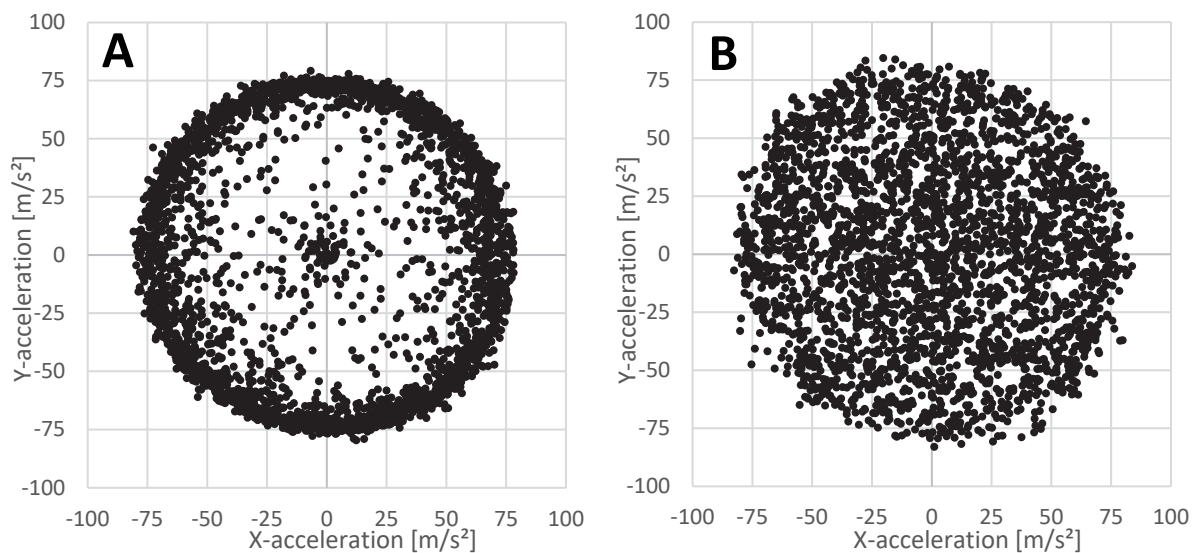
Figure 2: Measurement of acceleration in x- and y-axis at an unloaded milling run with 1400 rpm with sensor in (A) suitable measuring position according to figure 1 and in (B) unsuitable measuring position (near an attachment point of a horizontal spring) to evaluate the concentricity of the disc mill 10 .
