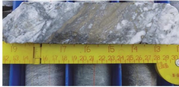
Figure 1. Length of strongly sulphide (late phase) mineralised core yielding a grade of 108 g/t Au over 0.2 m, typical of the VC. The other side of the core contained visible gold.
