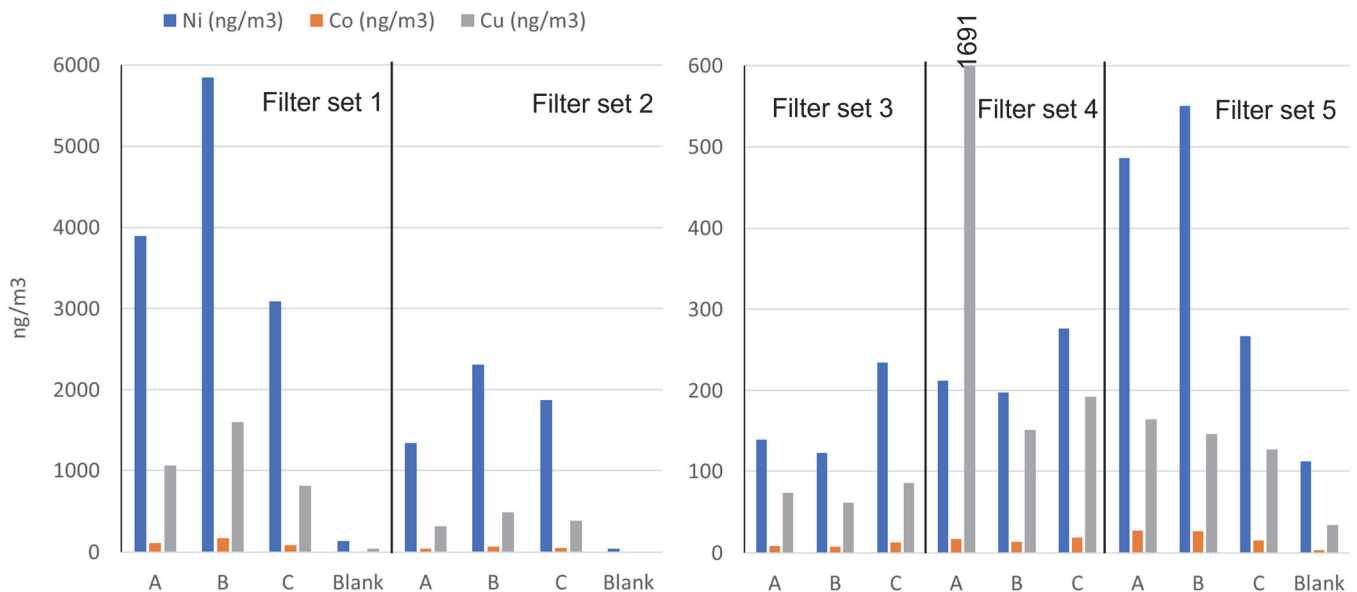
Figure 4. Overview of data from inter-comparison of Ni, Co and Cu concentrations from 3 filters in five sets of varying Ni mass. The blank is shown for 3 sets. Filter set 4 has one outlier.
