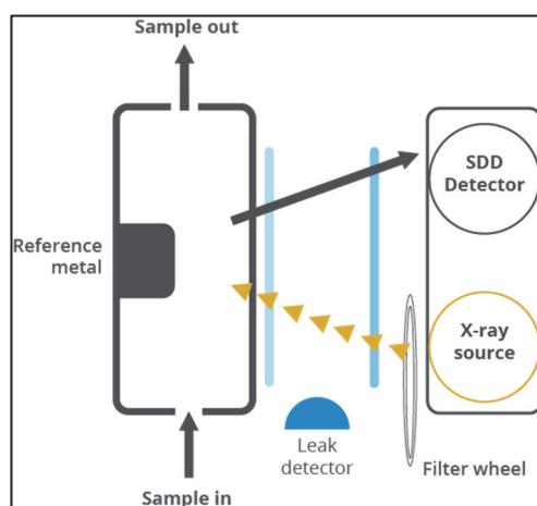
Figure 5. Hóbré C-Quand XRF analyzer cell layout.
