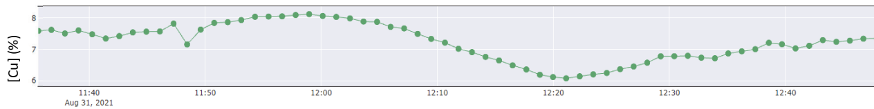
Figure 6. Evolution of the measured Cu concentration in a copper ore slurry over the course of an hour. The observed changes over time indicate the parameter changes of the process parameters performed during the flotation test, demonstrating the capability of online and inline monitoring of an elemental analyser for mineral preparation.
