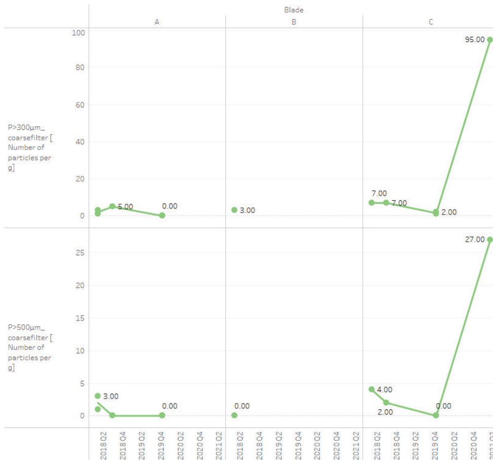
Figure 14.1 Trend data for blade bearings without sign of faults (very low and constant amount of large ferro-magnetic wear particles) and the bearing C with significantly increasing content of ferro-magnetic wear debris.
