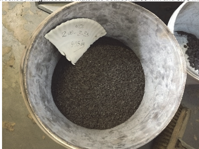
Figure 6: Closely screened manganese ore materials between 2.00 mm and 3.35 mm, with an average d_N = 2.659 mm The average nominal top-size of a fraction retained between screens of 1.266 cm and 0.63 cm is calculated as follows:
