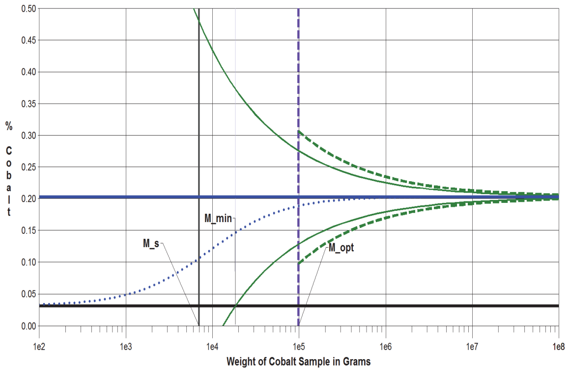
Figure 4. Calculation of the standard deviation s_{opt} illustrated as the dashed curves.
