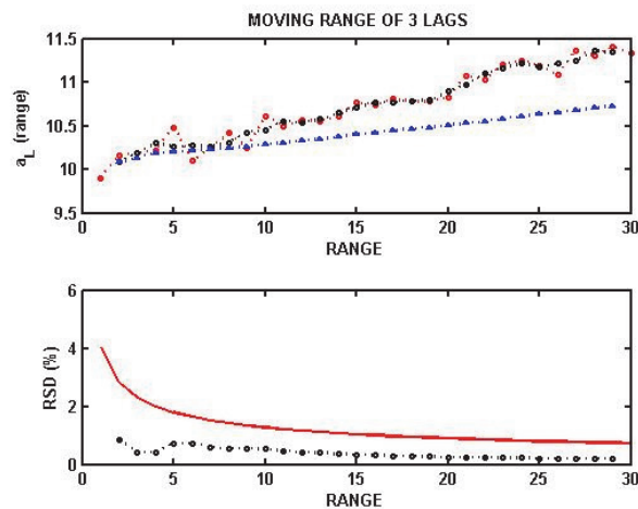
Figure 2. The upper panel shows 30 measurements from the simulated linear process (red dots) and mean of moving windows of 3 lags. The lower line shows the moving average as function of increasing range. The lower panel shows the relative standard deviation as a function of the number of measurements; the upper (red line) ignores the autocorrelation and in the lower panel the relative standard deviation is estimated with the current method from the consecutive moving windows of three measurements.
