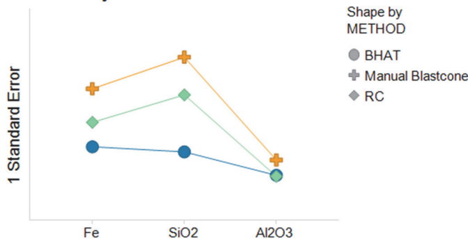
Figure 1. Summary results for different methods of assay data acquisition at a mining site (left). Note the high error for manual blastcone sampling using shovels and the lowest error for the BHAT method. The plot on the right shows field error for three BHAT units operating at the mine site, showing consistent results. Note: One Standard Error is given as the standard deviation of the absolute difference between sample pairs.
