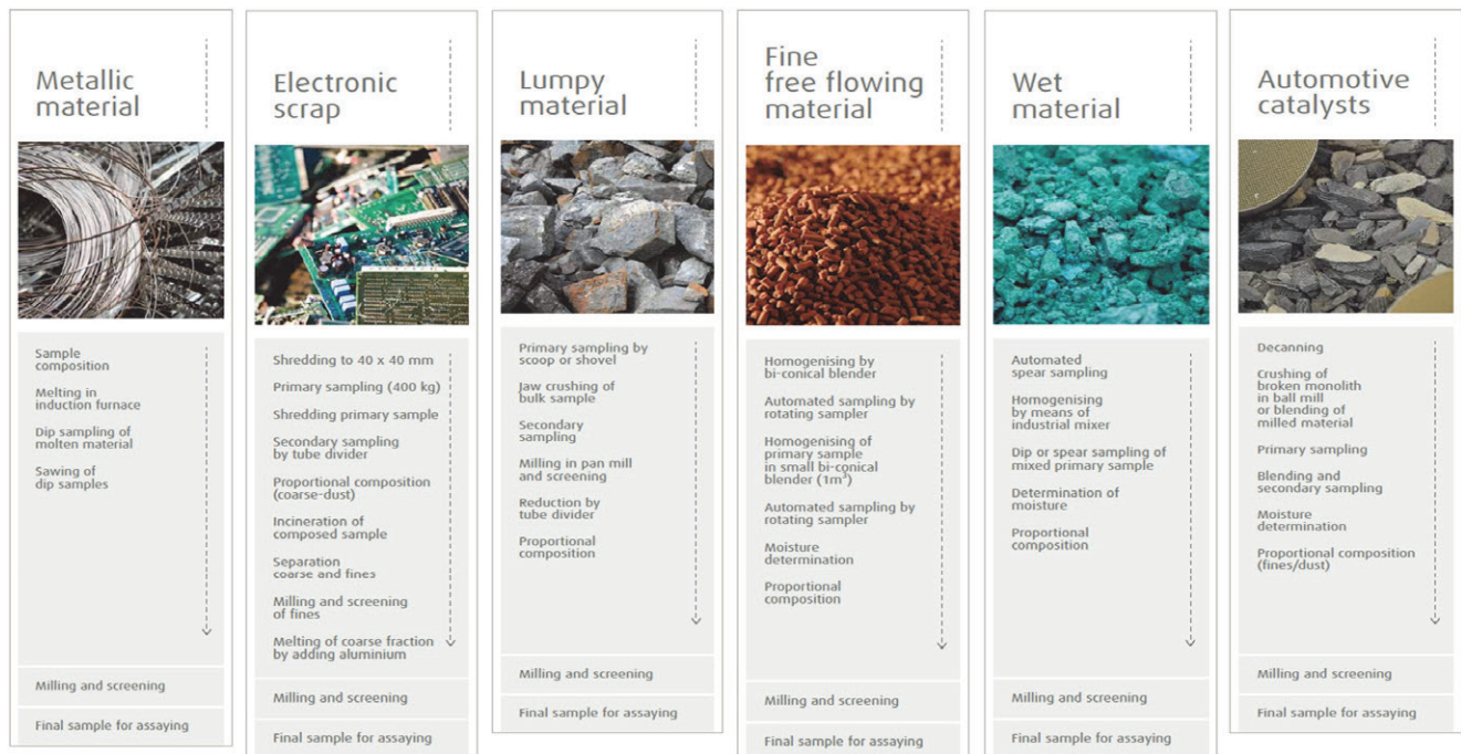
Figure 5. Dedicated Sampling Lines @UPMR
