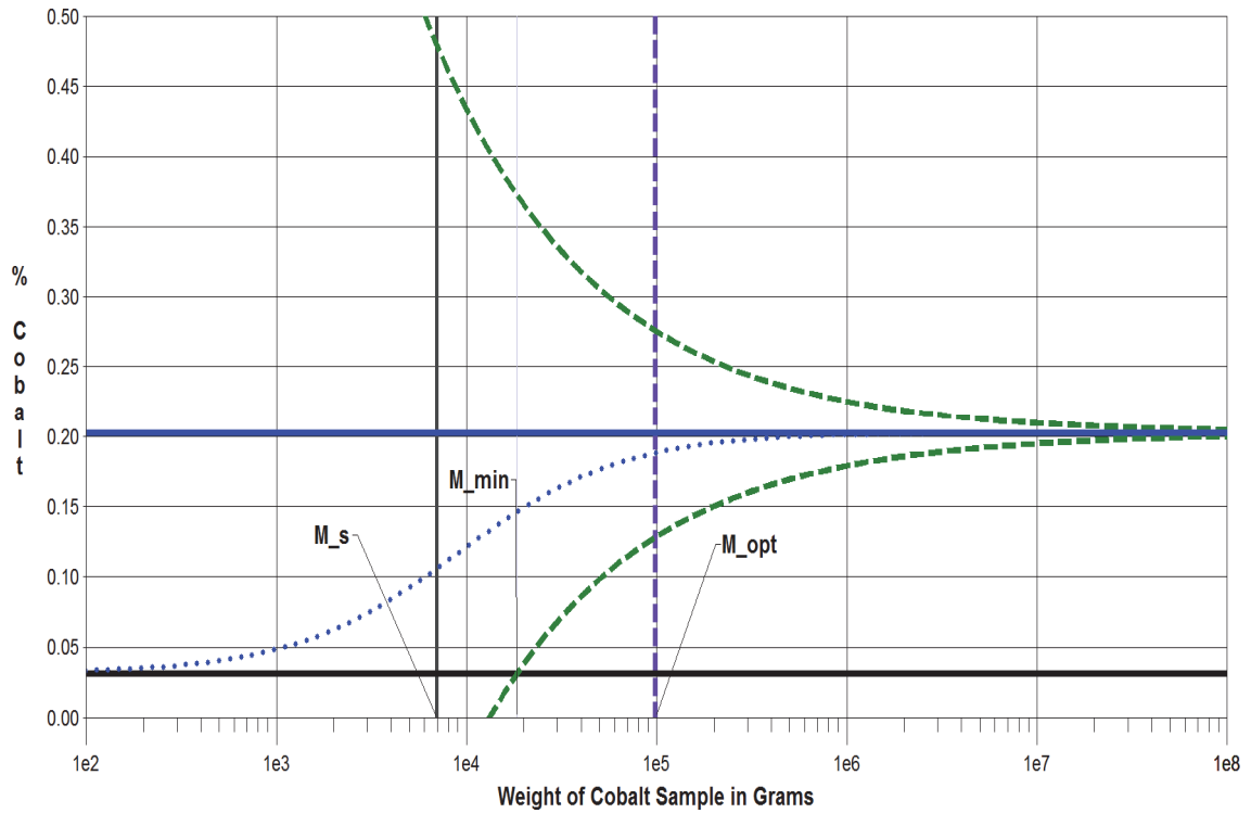
Figure 3. Calculation of the standard deviation s_{FSE} a_L
