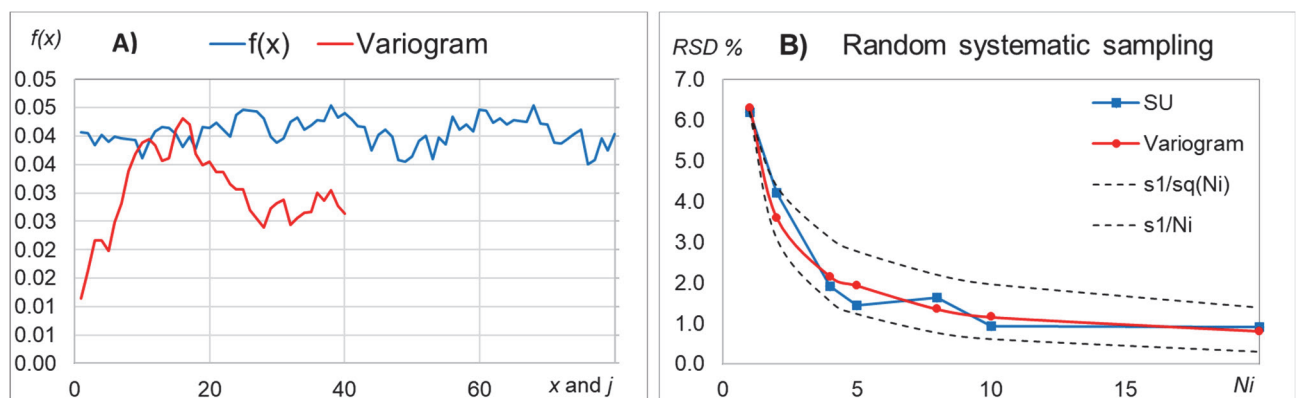
Figure 3. Data without trends (Slope( f(x) ) = 0). Predictions of sampling uncertainty (RSD %) for variogram integration and for SU estimation.
