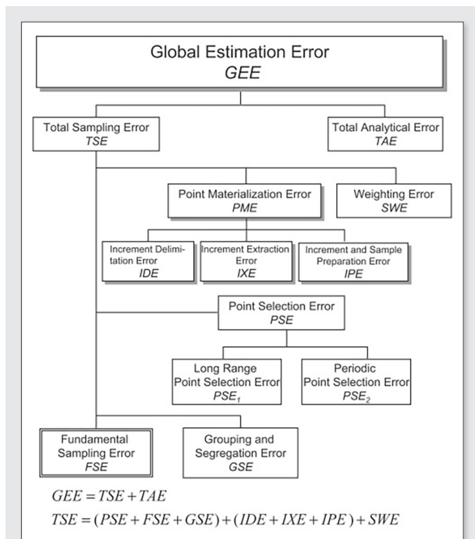
Figure 9. Gy's complete classification of sampling errors according to source 4 .
